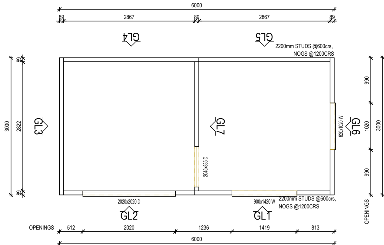
WALL FRAME LAYOUT
