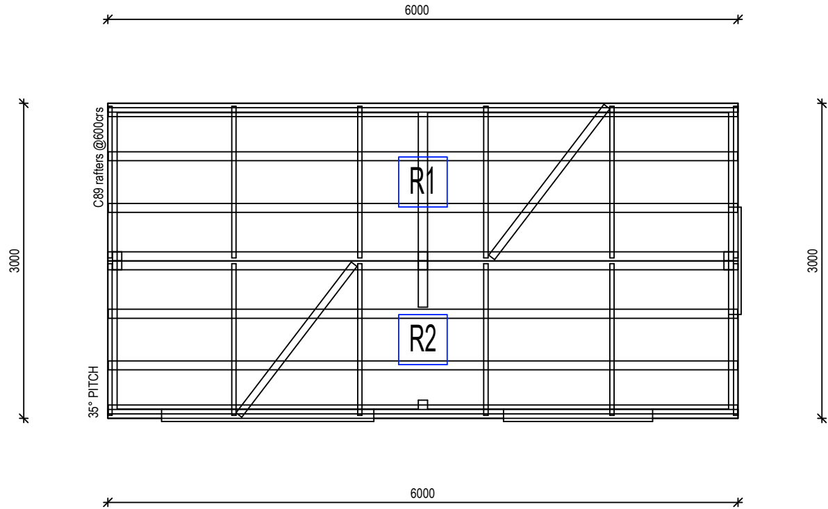
ROOF FRAME LAYOUT
